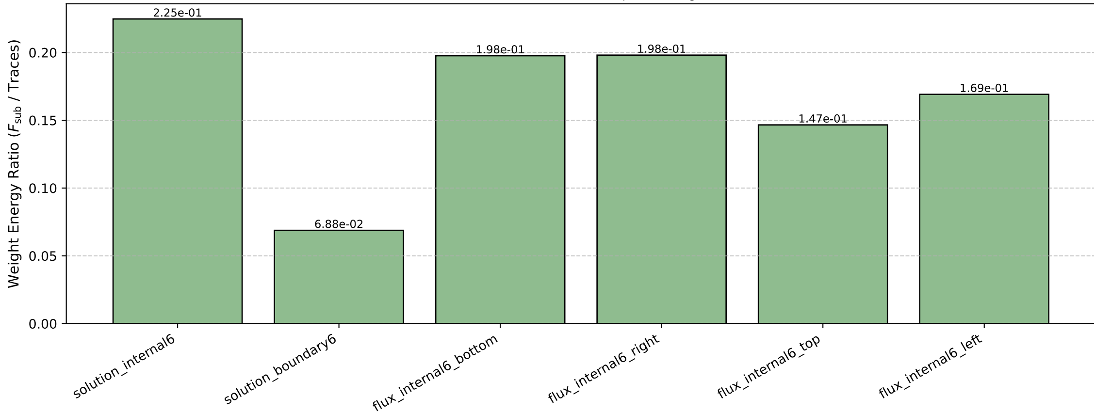
First Layer Sensitivity Ratio: \|W_F^{(1)}\|_2 / \|W_U^{(1)}\|_2 (Training 6)
