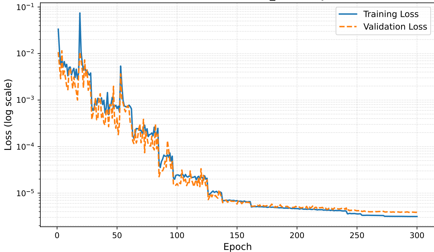
Loss Evolution: solution_boundary6
