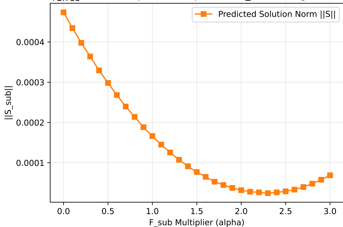
+2.735 Solution Operator Response to F_sub Scaling
