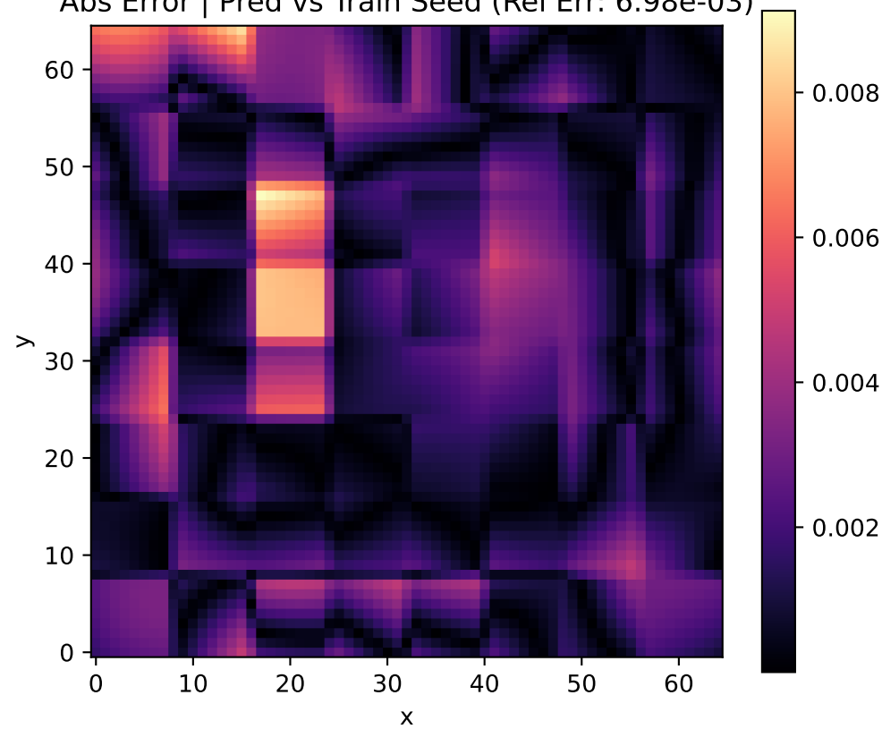
Abs Error | Pred vs Train Seed (Rel Err: 6.98e-03)
