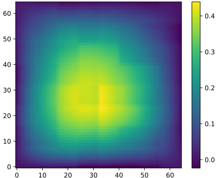
U-Net Prediction
