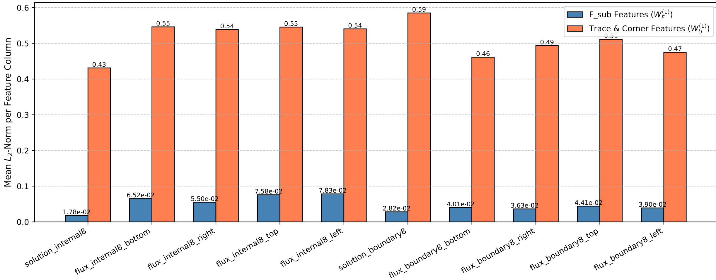
First Layer Weight Audit: Mean Column L_2 -Norm per Feature
