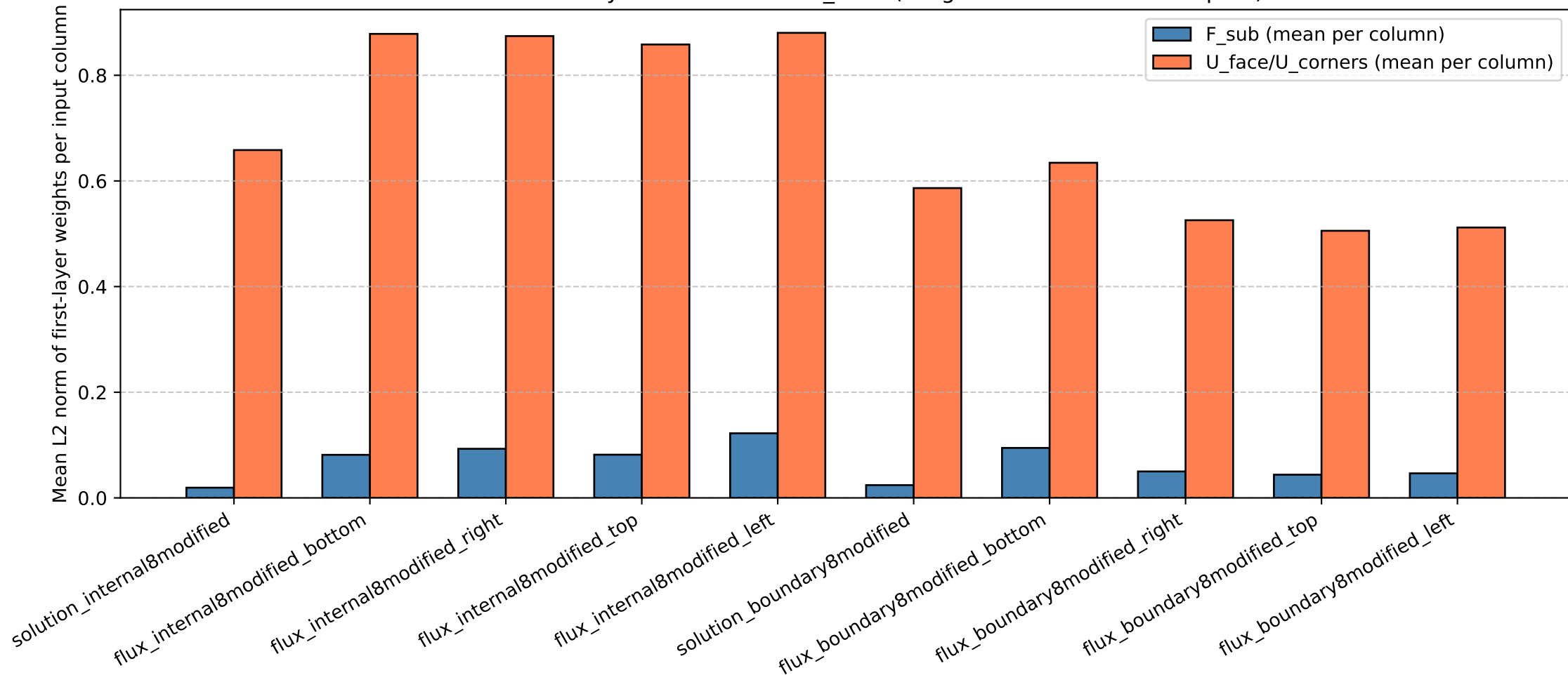
Does the first layer even listen to F_{\text{sub}} ? (weights on standardized inputs)
