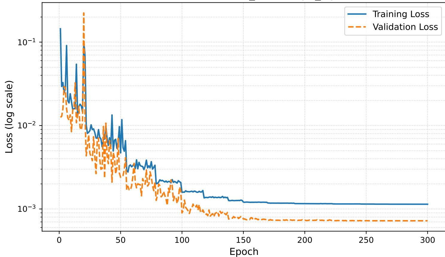
Loss Evolution: flux_boundary8_right
