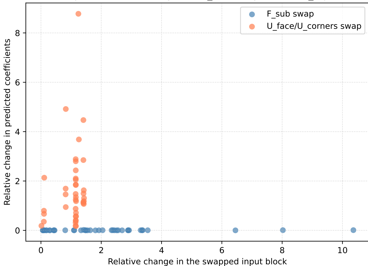
Input block sensitivity — flux_boundary8modified_top
