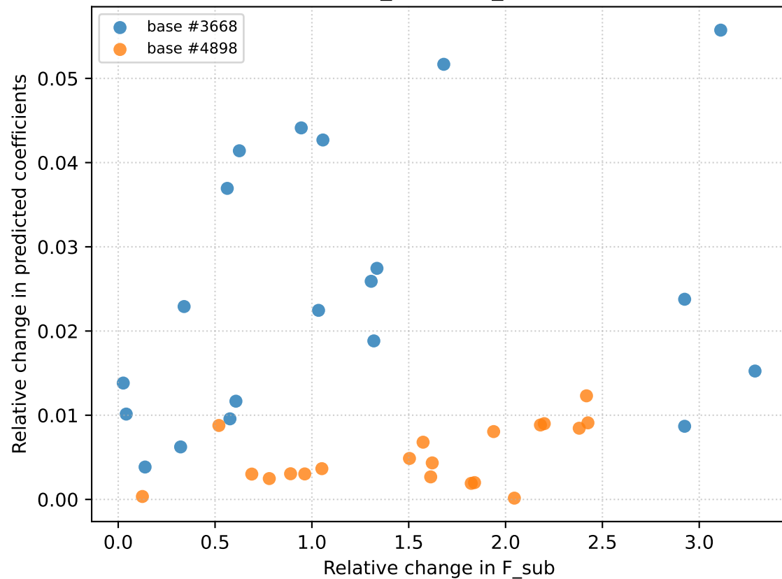
Coefficient sensitivity flux_internal8_left
