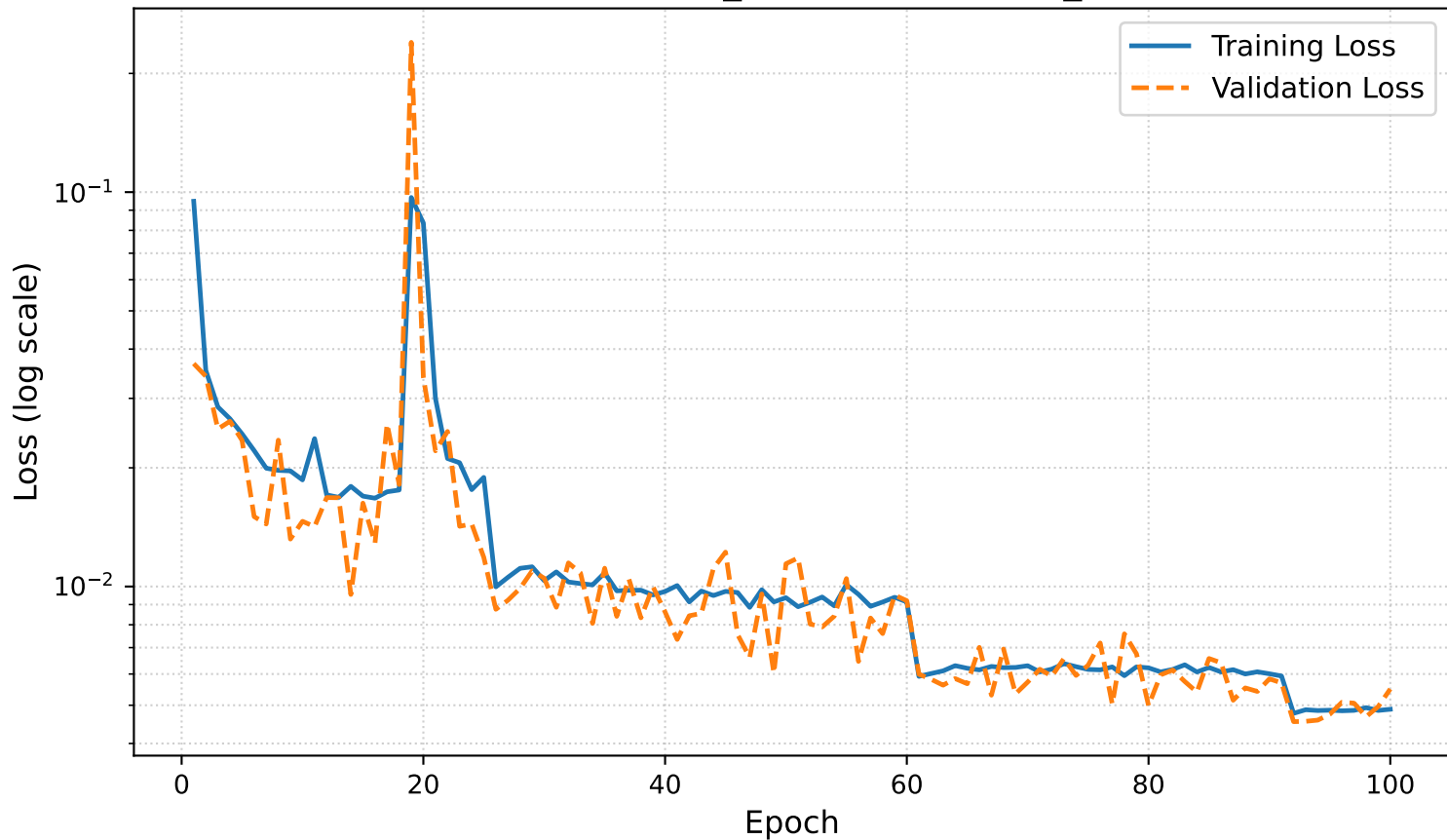
Loss Evolution: flux_internal8modified_bottom
