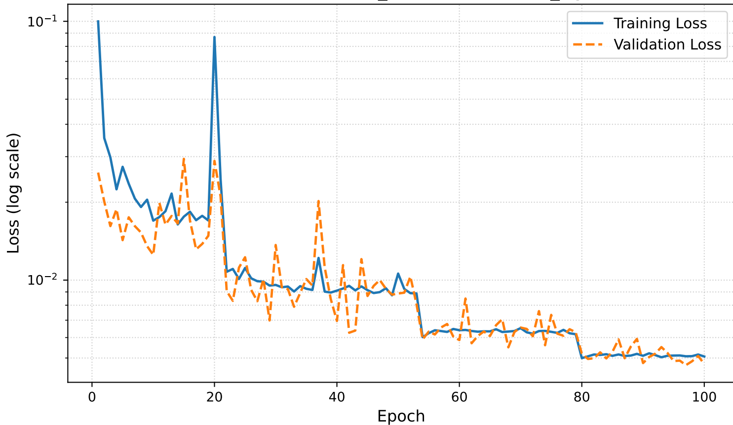
Loss Evolution: flux_internal8modified_right
