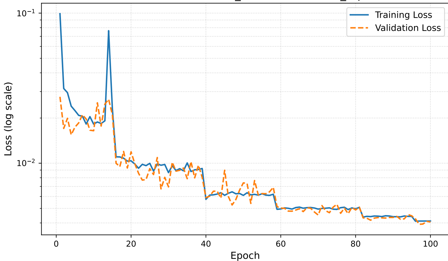
Loss Evolution: flux_internal8modified_top
