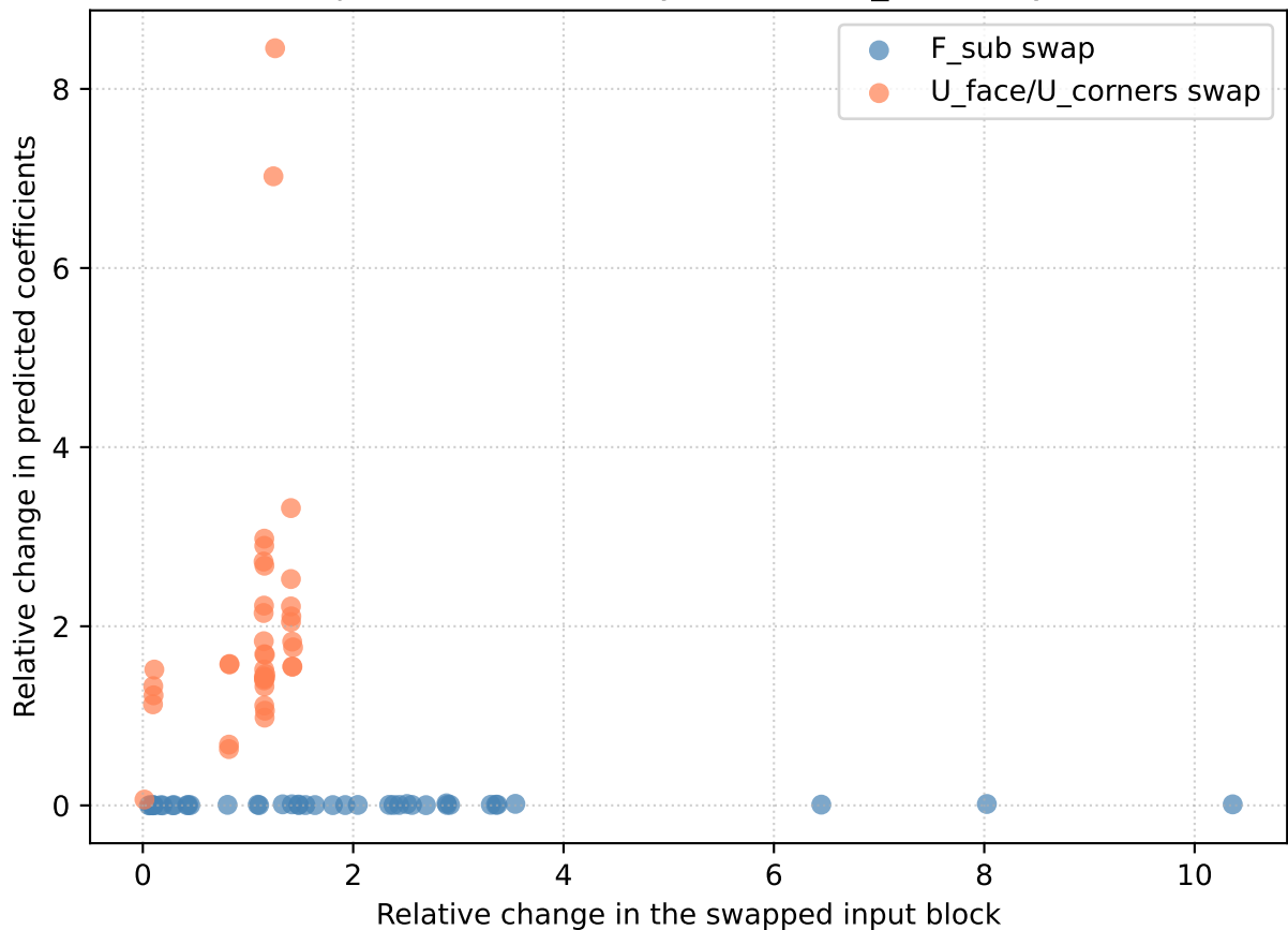
Input block sensitivity — solution_boundary8
