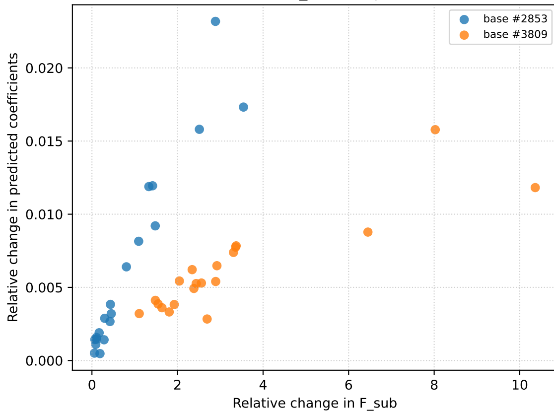
Coefficient sensitivity solution_boundary8
