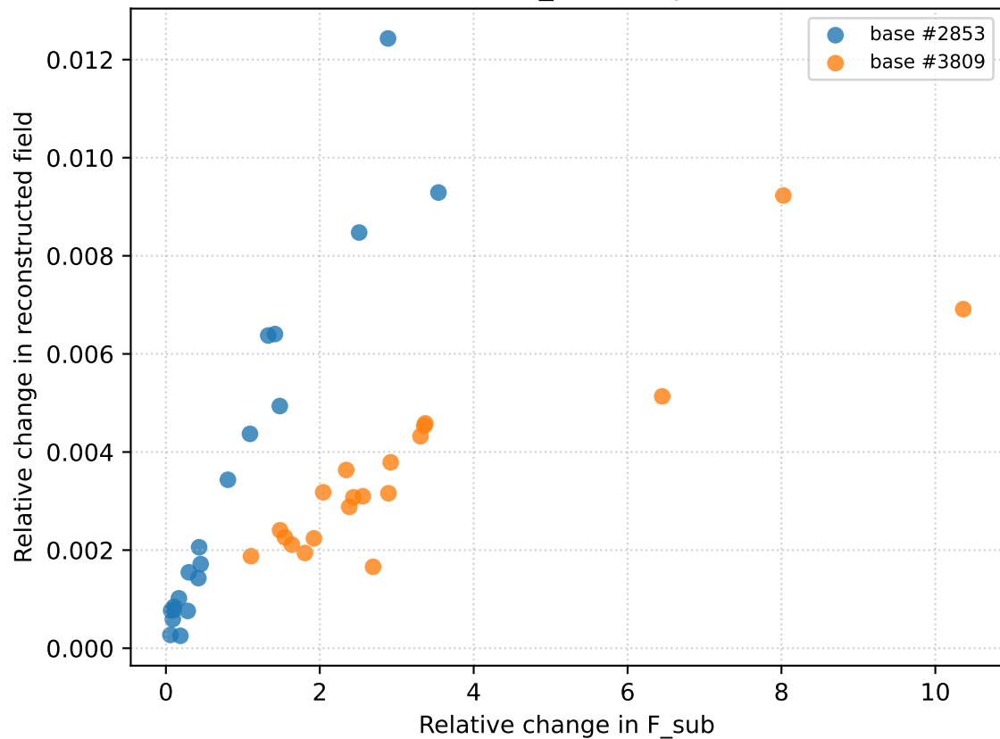
Physical field sensitivity solution_boundary8
