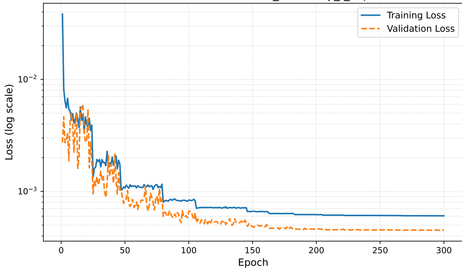
Loss Evolution: solution_boundary_f_sep
