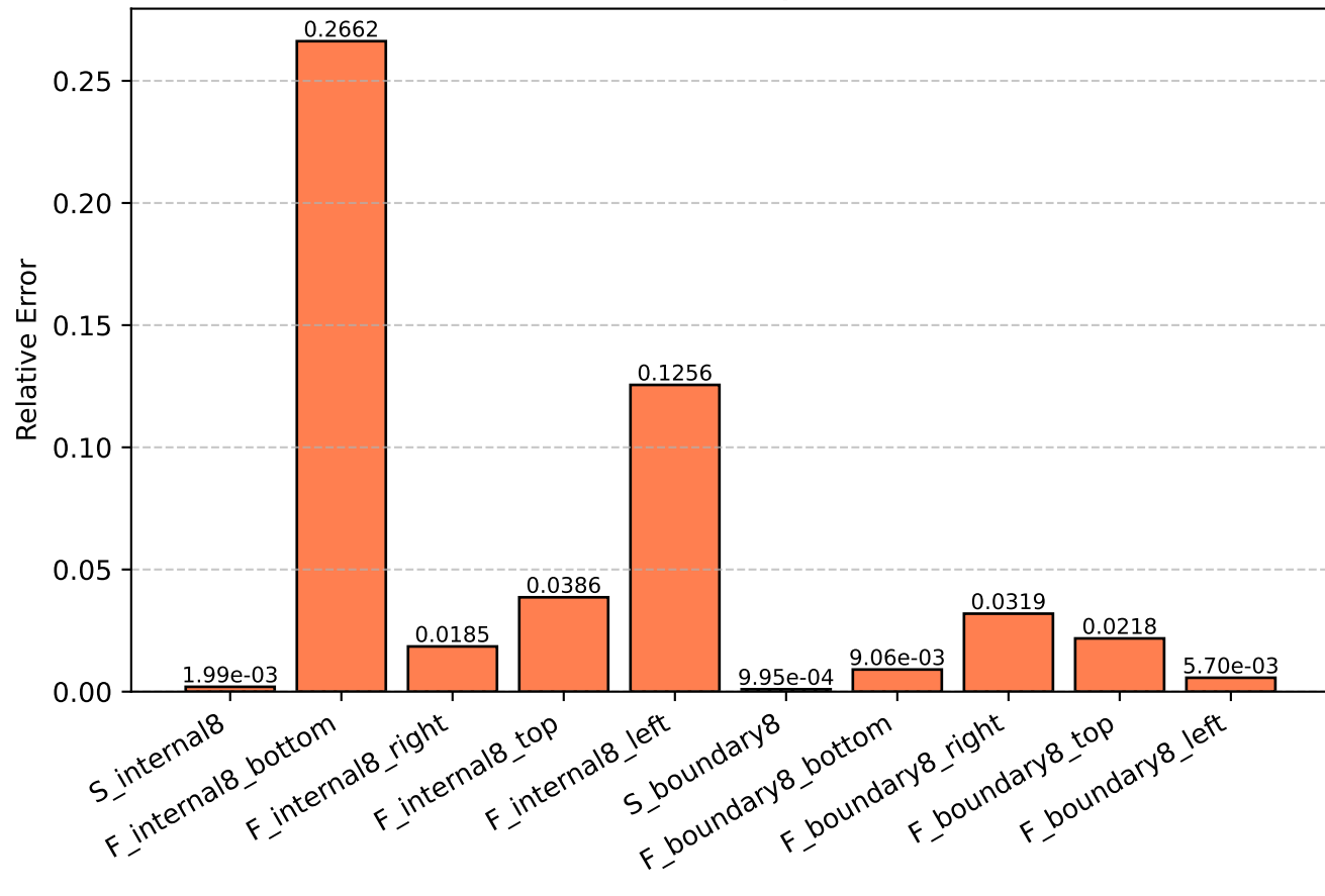
Relative Error by Operator
