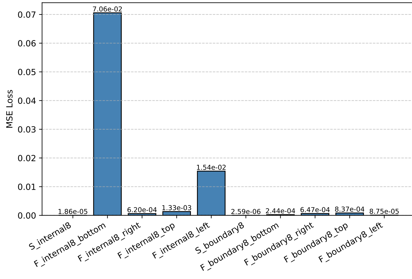
Test MSE by Operator
