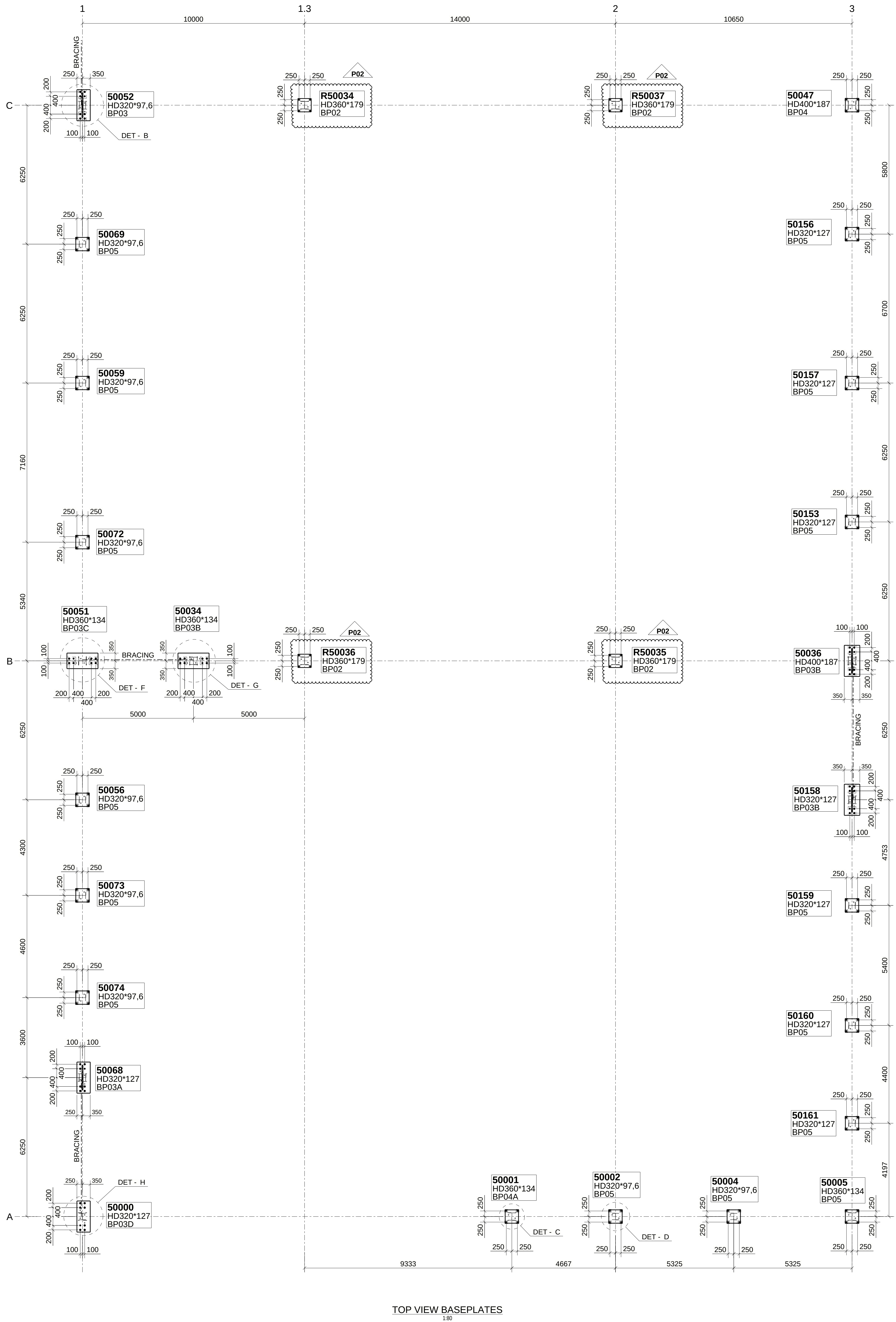
TOP VIEW BASEPLATES 1:50
