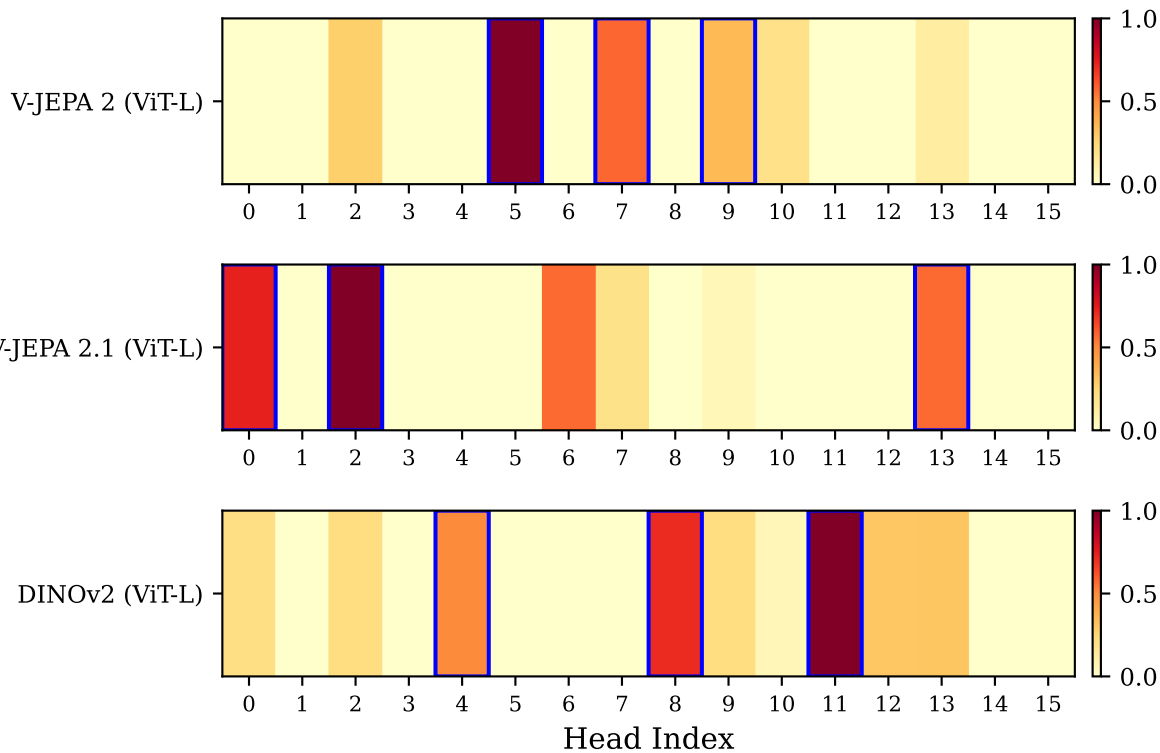
Per-Head Affordance Importance at Peak Layer (Blue box = top-3 heads)
