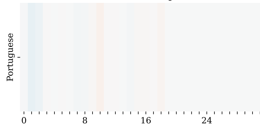
Attention Output
