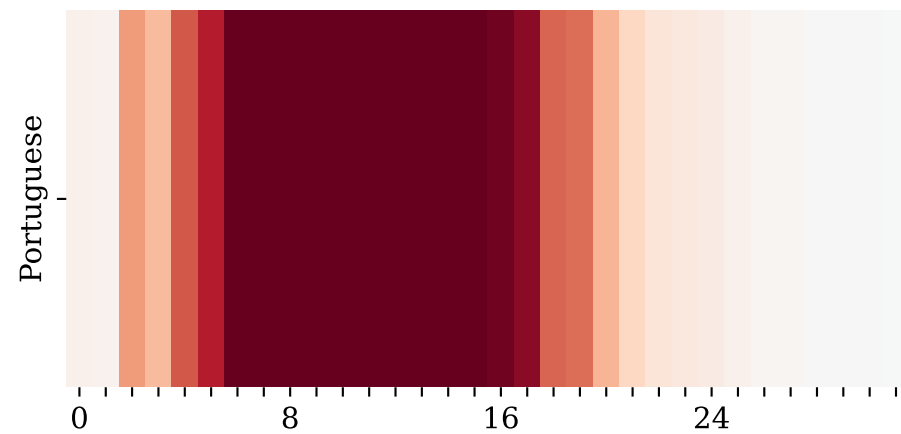
Residual Stream
