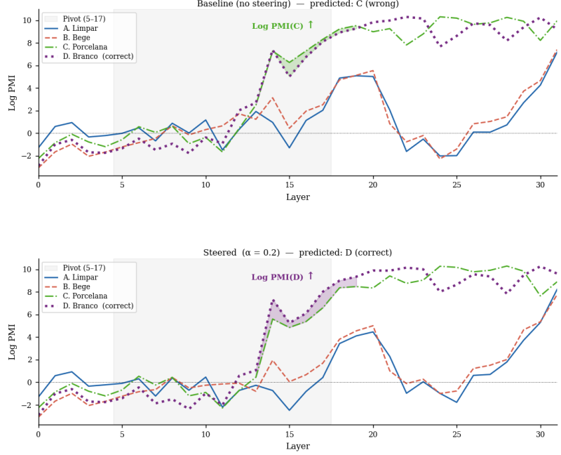
Figure 4: Representative Portuguese MMMB case (steered wins). Left: input image and question with four answer options; correct answer is D. Top right (Baseline): logit-lens PMI curves for all four options across 32 layers—the model incorrectly peaks on option C at layer 31. Bottom right (Steered, \alpha=0.2 ): after applying the Portuguese steering vector at pivot layers 5–17, option D dominates at layer 31, recovering the correct answer. The shaded fill in the pivot region highlights where C and D compete; steering resolves this competition in favour of the correct option.
