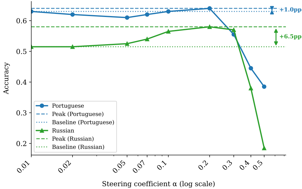
Figure 5: Sensitivity to steering coefficient \alpha on MMMB. Performance peaks at \alpha=0.2 and degrades sharply beyond \alpha=0.3 . The effective window ( \alpha \in [0.05, 0.2] ) is consistent with prior representation-engineering results (Zou et al., 2023).
