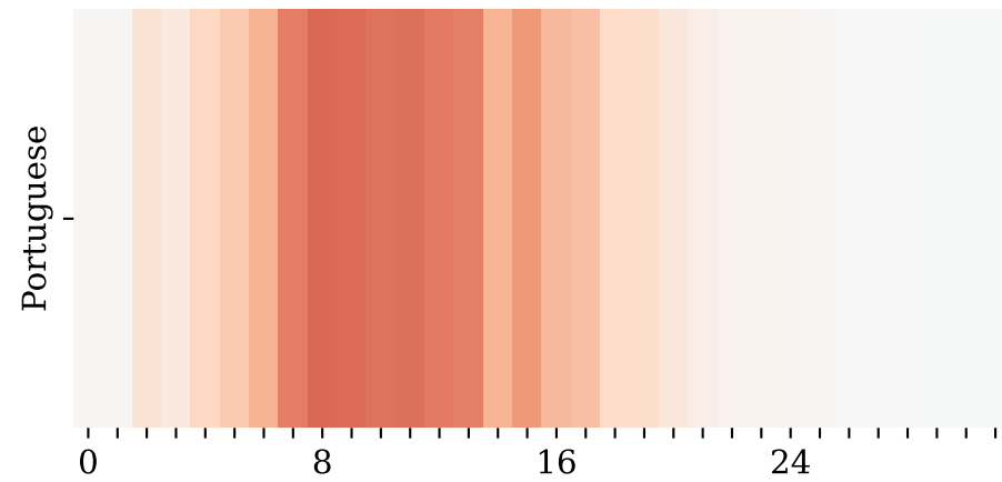
Residual Stream
