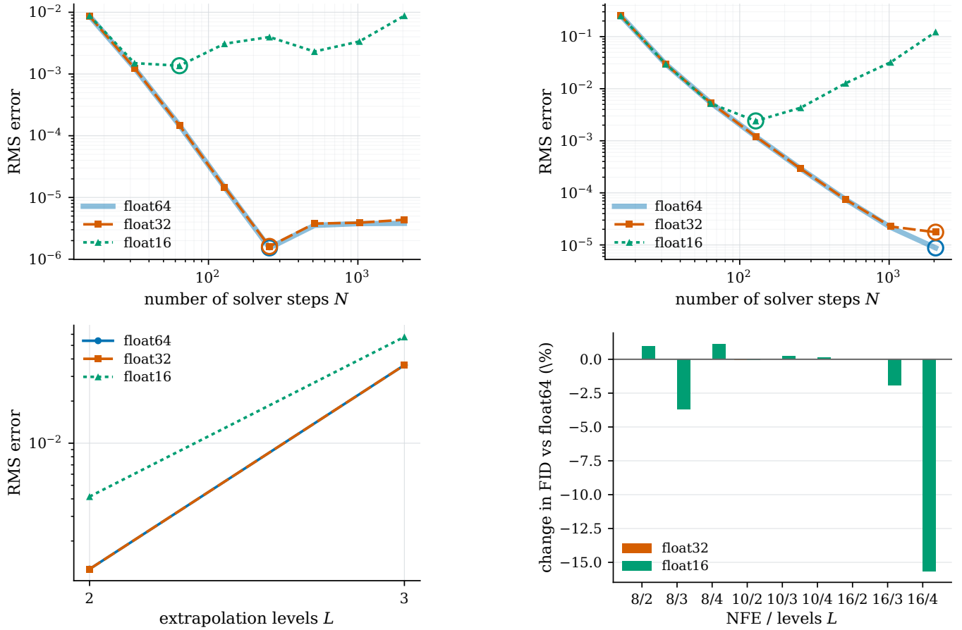
Figure 9: Truncation error against round-off error. Upper row: RMS error against the number of solver steps at two levels (left) and three levels (right), for three working precisions of the extrapolation arithmetic, with open circles marking the minimum of each curve. Lower left: RMS error against the number of levels, which increases monotonically. Lower right: change in FID relative to double precision on CIFAR-10, by budget and level count.
