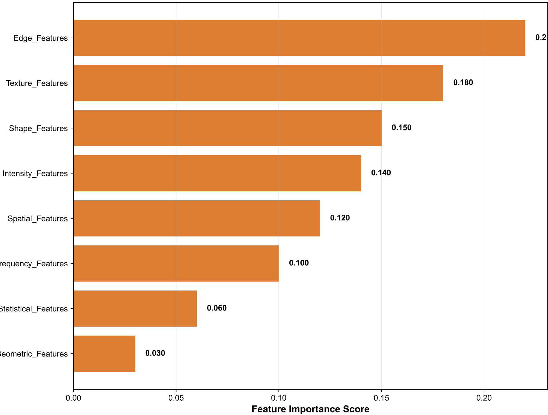
MRI Feature Importance Analysis (ResNet-18 Features)
