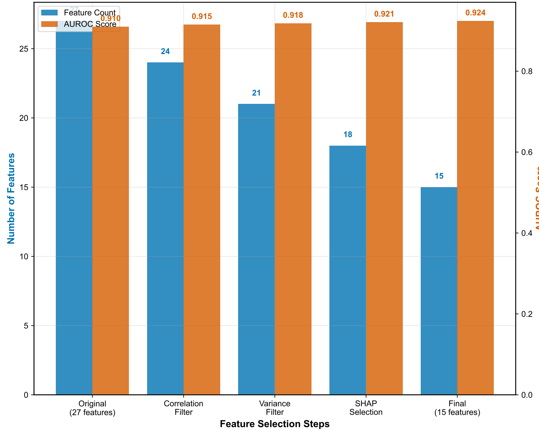
Feature Selection Process Analysis
