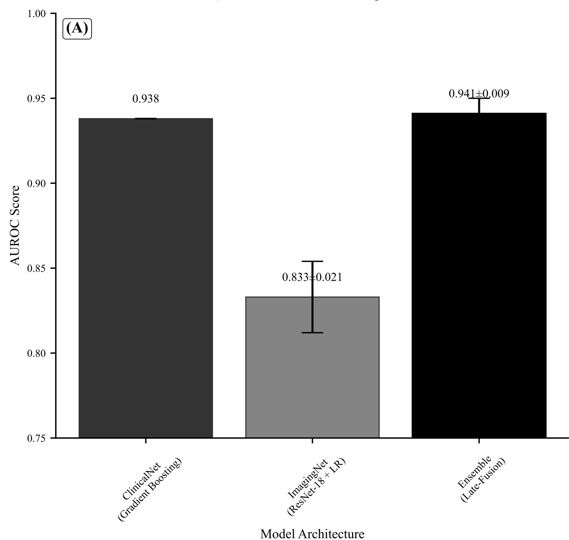
A) Model Performance Comparison
