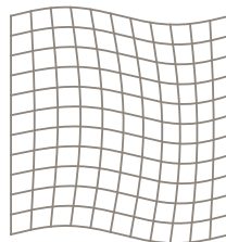
Invertible
