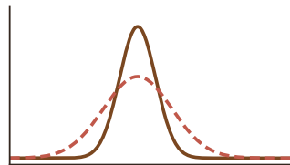
Extent
