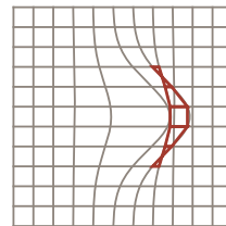
Folded
