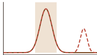
Support
