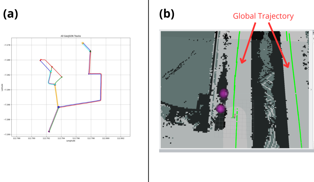
Figure 7.8. Result of Global Navigation Estimation
