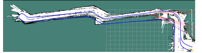
Fig. 4. Occupancy grid map generated using wheels and IMU odometry.
