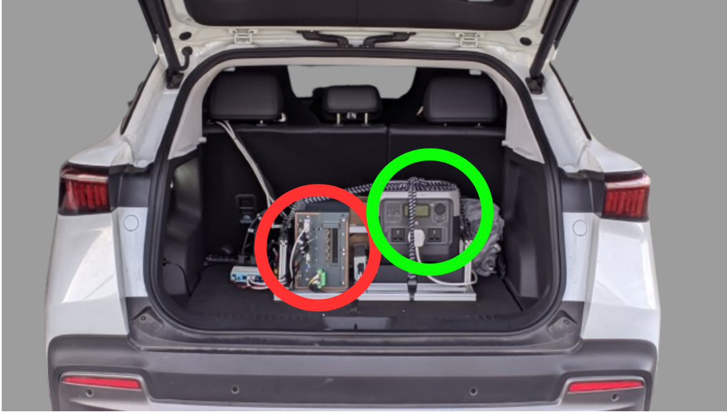
Figure 7.2. Computing Hardware
