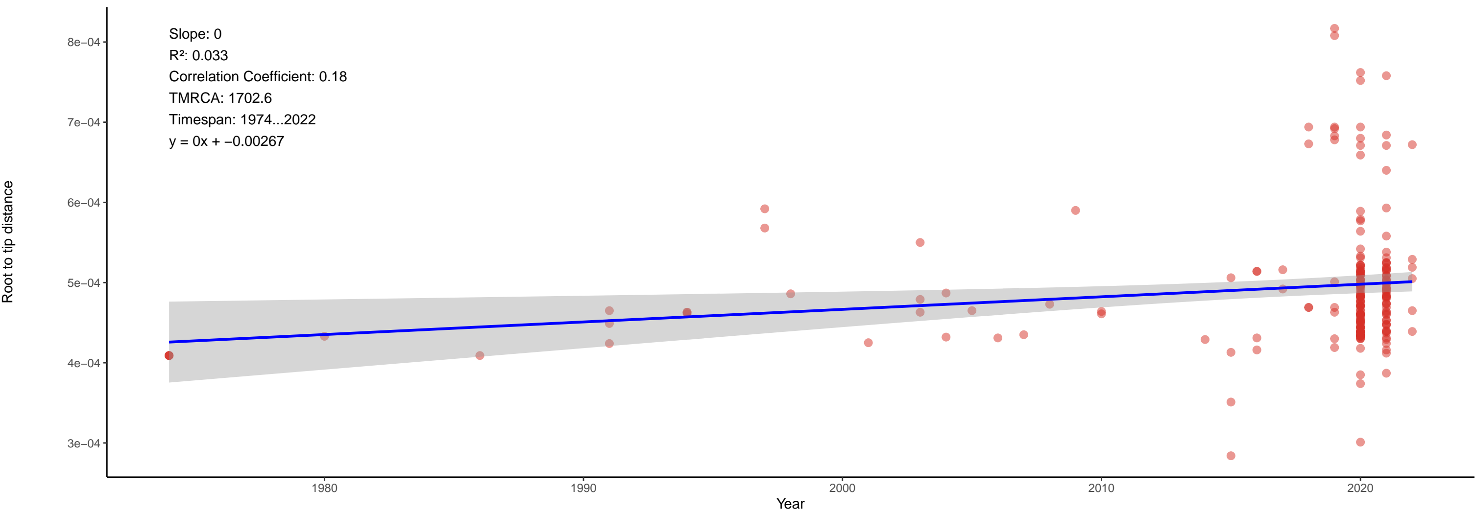
A.Root to tip distance plot to evaluate temporal signal
