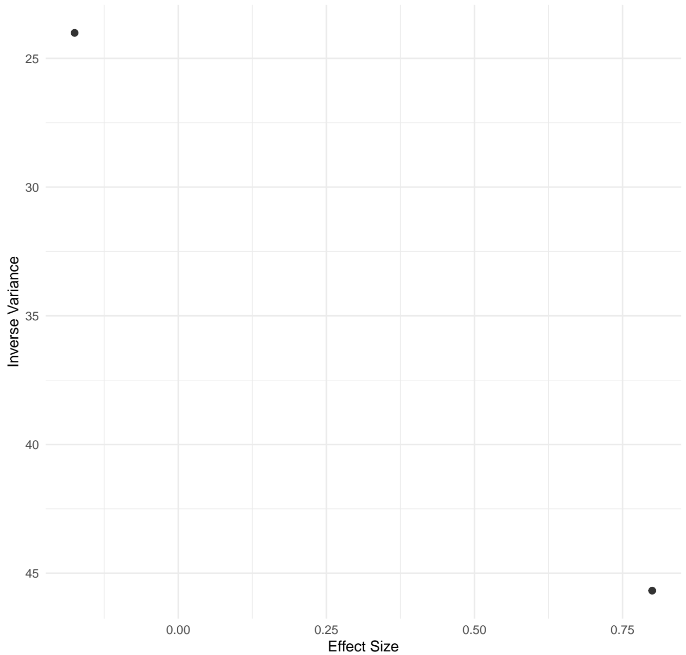
Effect Size vs Precision – 4 | Health & access disparities
