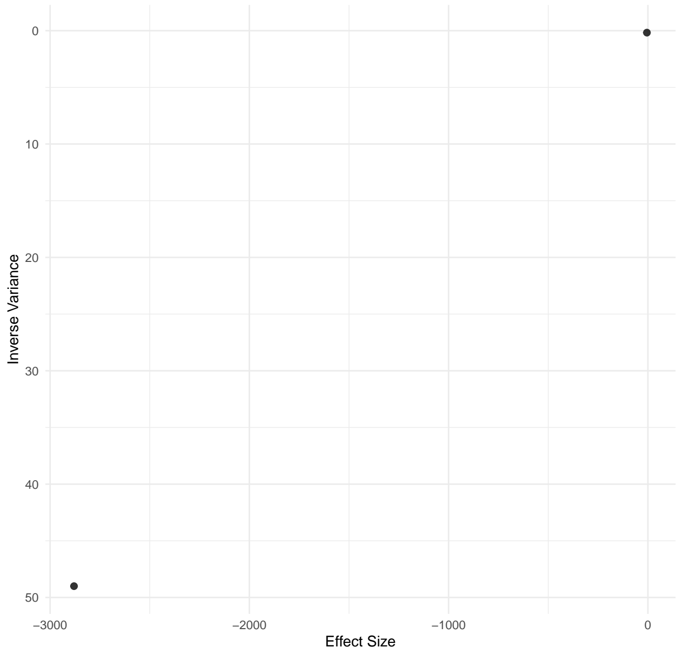
Effect Size vs Precision – 3 | Health System Performance
