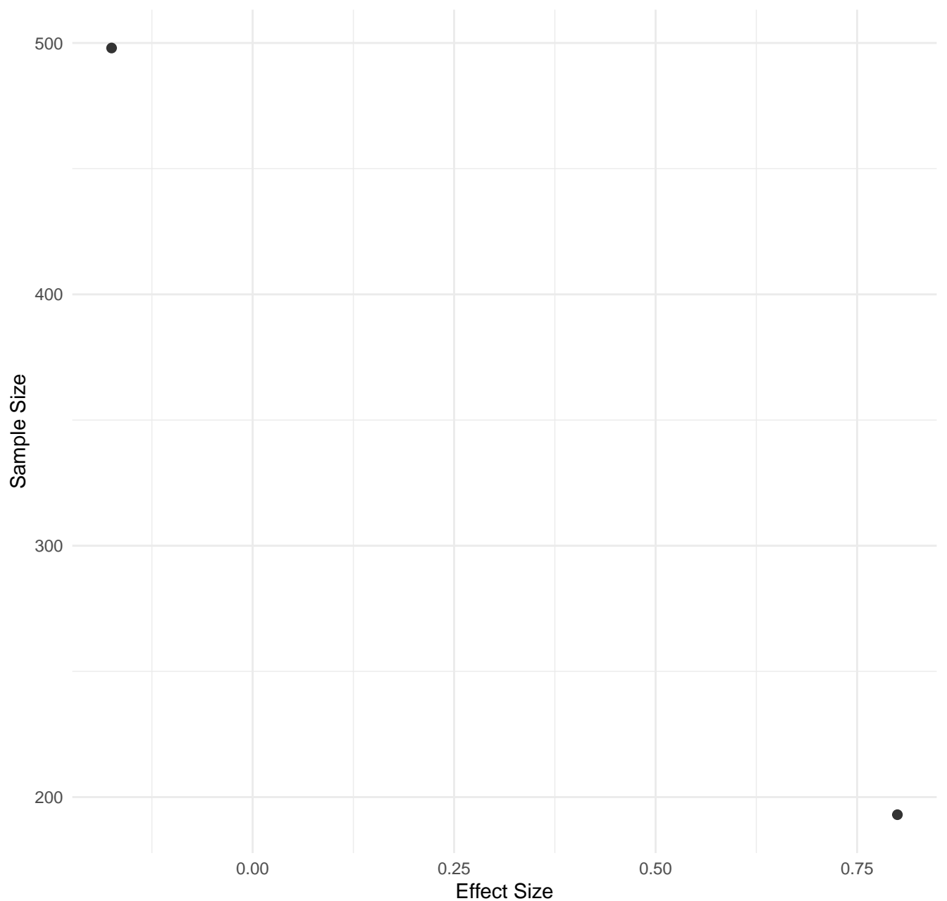
Effect Size vs Sample Size – 4 | Health & access disparities
