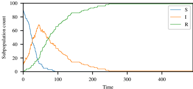
Simulated Disease Progression from SIR Model
