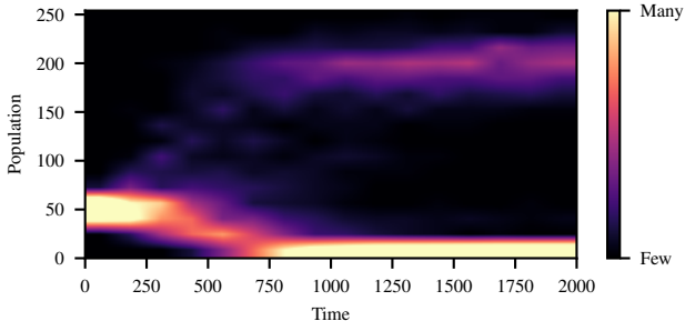
Simulated Populations with Allee Effect
