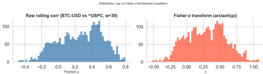
Figure 15: Distribution of the 30-day rolling correlation before and after Fisher-z transformation for the Bitcoin–S&P 500 pair. The transformation improves normality and removes boundary compression.
