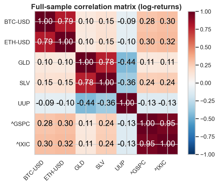
Figure 8: Static correlation heatmap of the return series.
