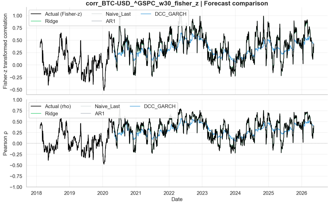
Figure 2: Observed and predicted Fisher-transformed dependency for the Bitcoin–S&P 500 pair at the 30-day rolling window. Forecast series are generated under strict walk-forward evaluation with no use of future information.
