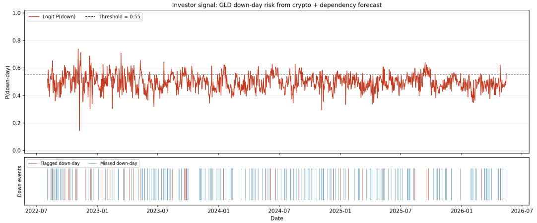
Figure 27: Signal-layer output for the Bitcoin–gold relation at the 30-day window.
