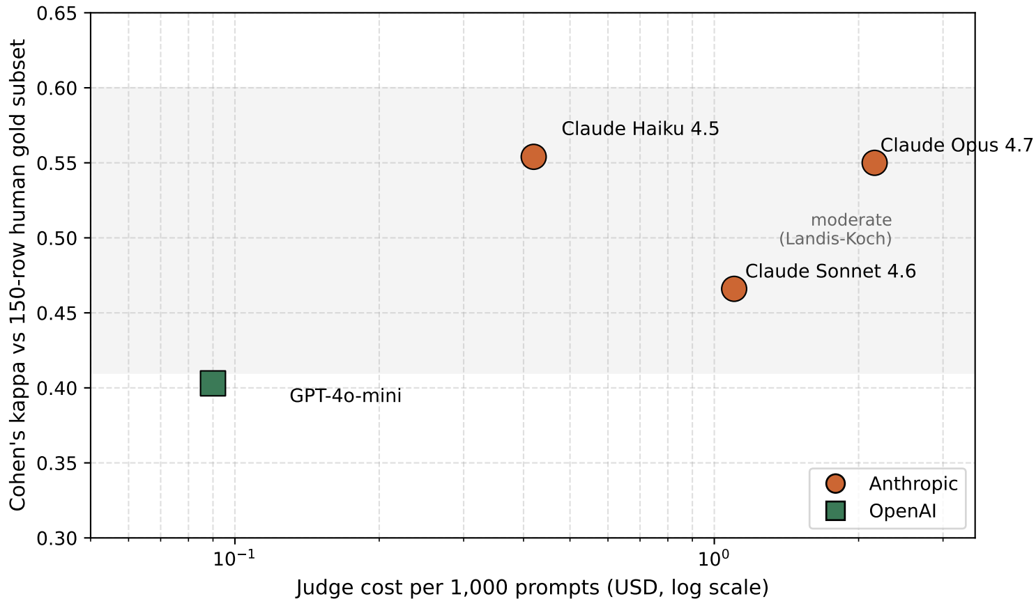
Judge reliability vs cost (v1.25 rubric, 150-row gold subset) Haiku 4.5 matches Opus 4.7 at one-fifth the cost
