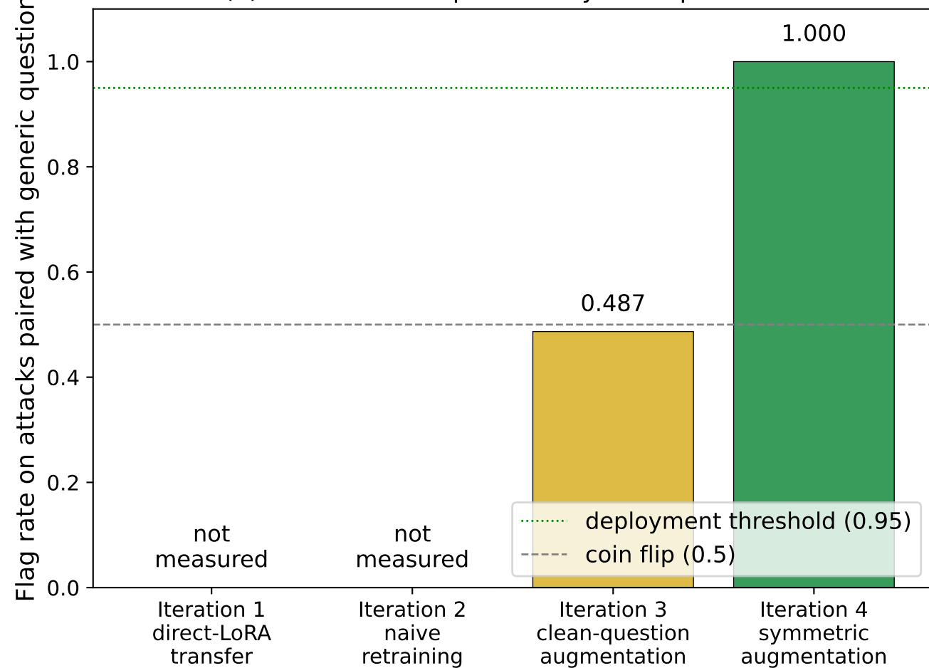
(b) Pressure test: question-style independence
