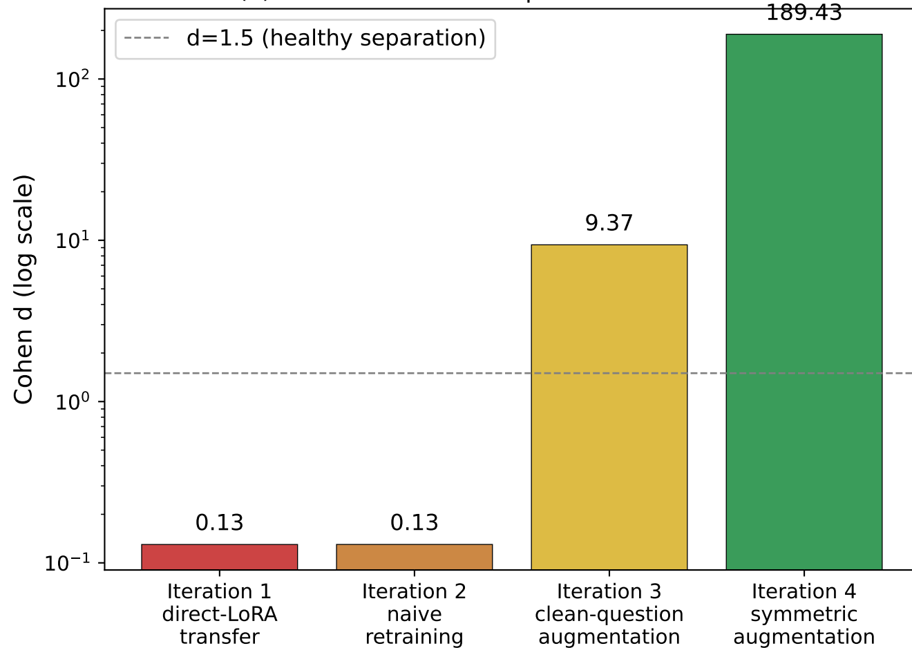
(a) Score distribution separation on BIPIA test
