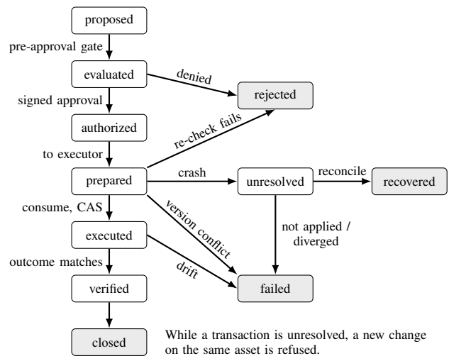
Fig. 2. Transaction states of the reference implementation; shaded states are terminal. A transaction is prepared when it is handed to the executor, which re-evaluates (1) and, only if all conjuncts hold, durably consumes the approval together with a journal entry, performs the controlled operation, and applies the compare-and-set (CAS); the signed receipt makes the transaction executed. The re-check edge also covers an approval that has already been consumed. The version-conflict edge also covers an approval that expires before the apply commit and a failure of the controlled operation. A crash after consumption and before the receipt leaves the transaction unresolved. After a late receipt the outcome is observed independently before the transaction is marked recovered; a mismatch ends it as failed. Every terminal state, and an unresolved state when archived, yields a signed envelope and a checkpoint.
