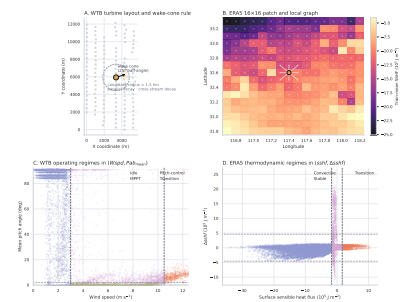
Fig. 1. Operating-decision context and physical regime anchors: (A) WTB layout with wake cone geometry; (B) ERA5 patch with sensible heat flux; (C) WTB operating regimes in ( W_{\text{spd}}, P_{\text{ab,mean}} ) plane with MPPT-to-pitch boundary; (D) ERA5 thermodynamic regimes in ( sshf, \Delta sshf ) plane.
