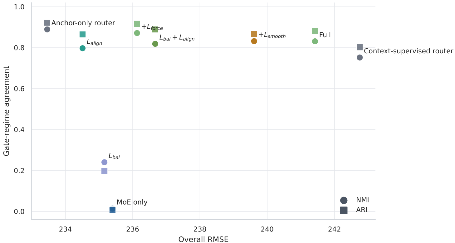
WTB accuracy-semantics tradeoff across routing variants
