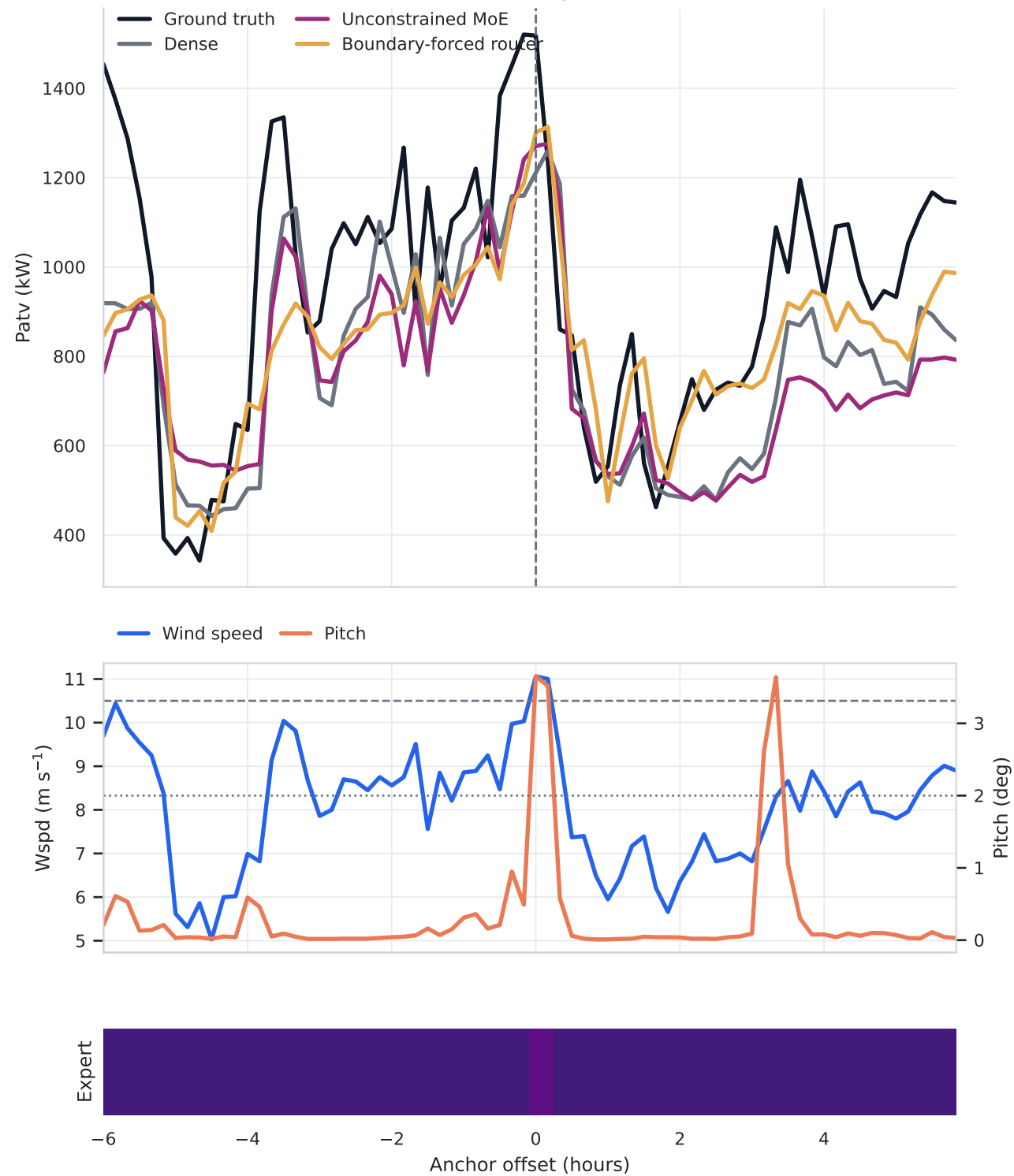
A. WTB local switch-window forecast comparison
