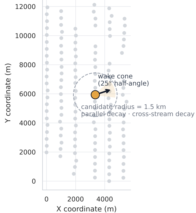
A. WTB turbine layout and wake-cone rule
