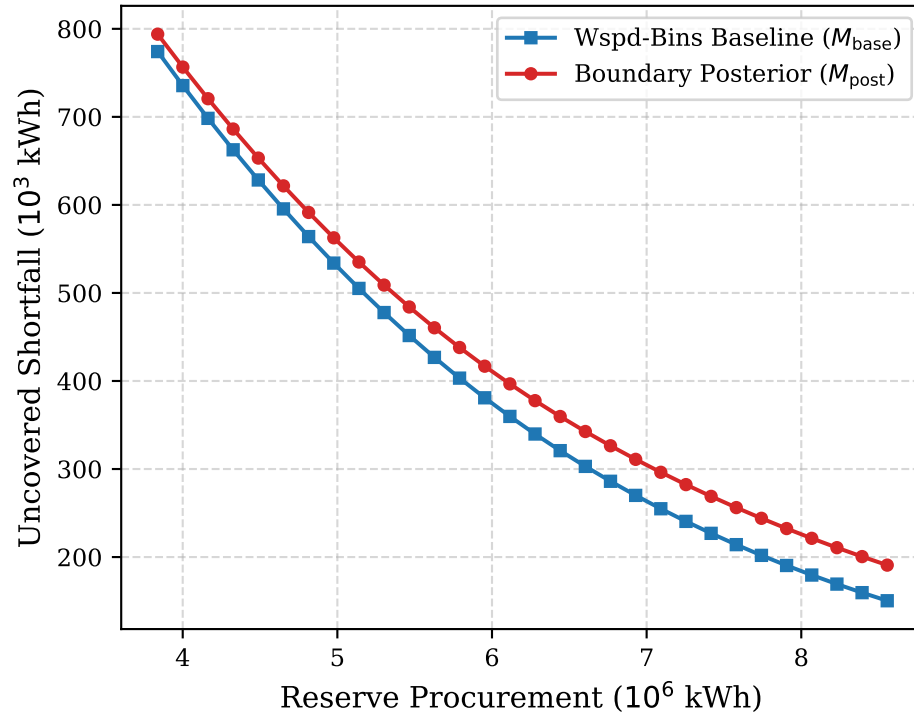
Negative Control: Stationary Window
