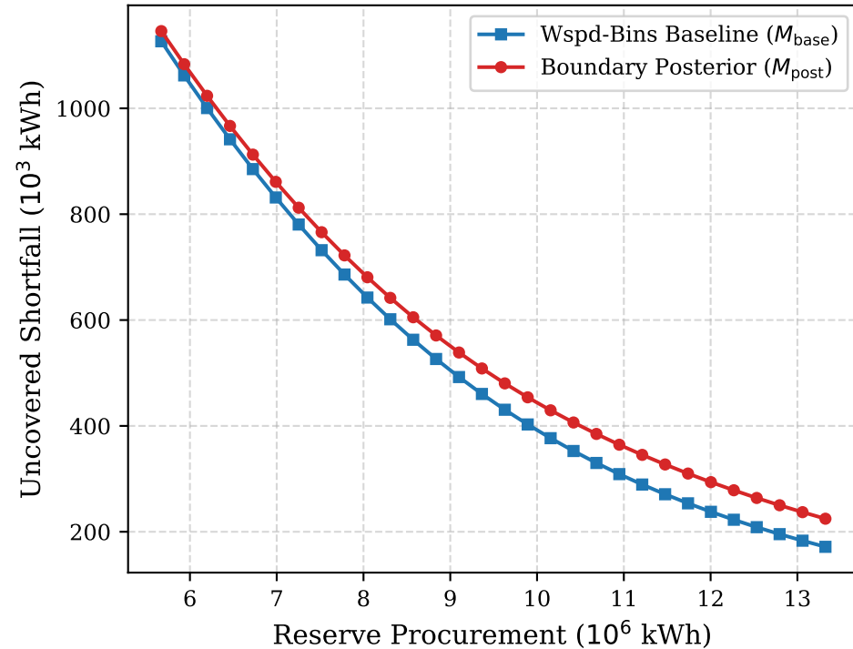
Global Control: Full Wind Farm
