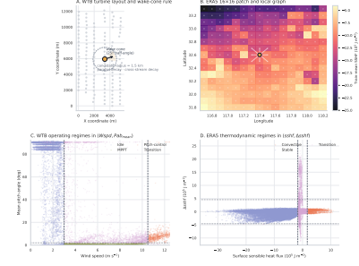
Fig. 1. Operating-decision context and physical regime anchors: (A) WTB layout with wake cone geometry (25° half-angle); (B) ERA5 patch with sensible heat flux; (C) WTB operating regimes in ( Wspd , Pab_{\text{mean}} ) plane with MPPT-to-pitch boundary; (D) ERA5 thermodynamic regimes in ( sshf , \Delta sshf ) plane.
