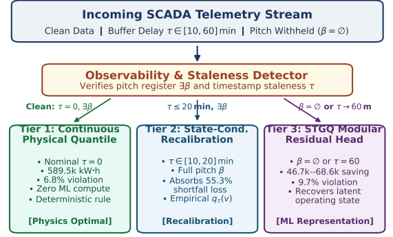
Fig. 1. Three-tier operational response logic under SCADA telemetry degradation: incoming telemetry streams are evaluated by an observability detector and routed to Tier 1 continuous physical quantiles under clean conditions, Tier 2 state-conditional recalibration under full-observability transmission latency, or Tier 3 STGQ modular residual quantile regression when blade pitch is unobservable or severe communication staleness breaks physical recalibration.
