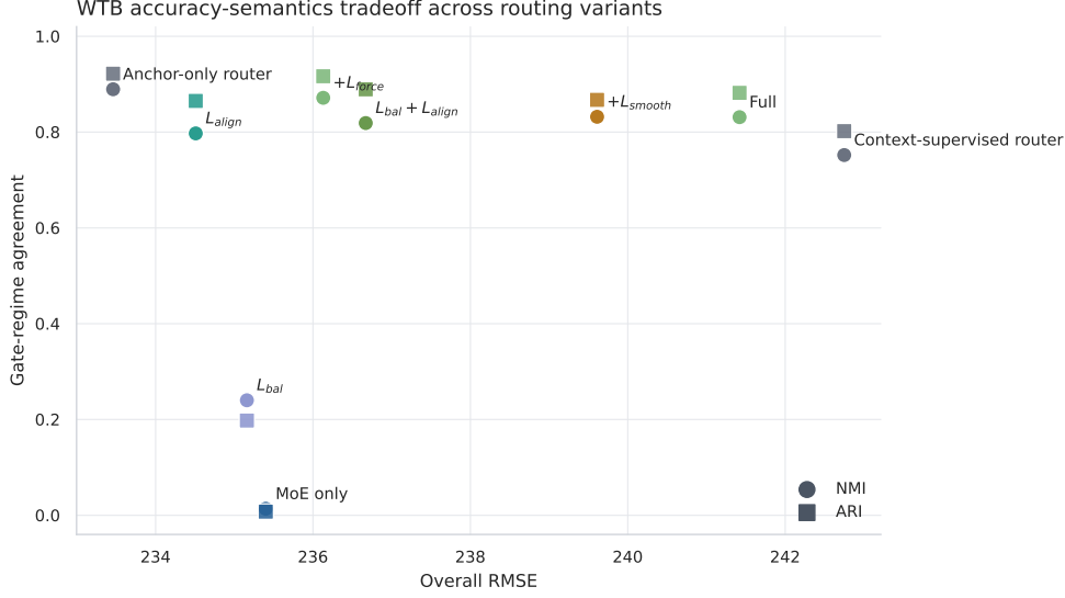
Figure 8: WTB accuracy-semantics tradeoff across routing variants. Circles show NMI and squares show ARI against overall RMSE. The frontier clarifies that stronger routing correction improves gate-regime agreement but can move the model away from the lowest forecast error.
