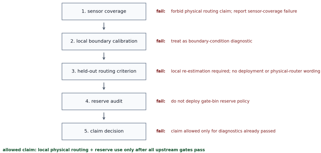
Figure 9: New wind-farm evidence protocol. The protocol moves from sensor coverage to local boundary calibration, held-out routing, reserve audit, and finally allowed or forbidden claims.
