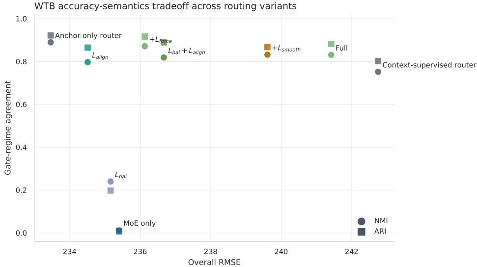
Figure 8: WTB accuracy-semantic tradeoff across routing variants. Circles show NMI and squares show ARI against overall RMSE. The frontier clarifies that stronger routing correction improves gate-regime agreement but can move the model away from the lowest forecast error.
