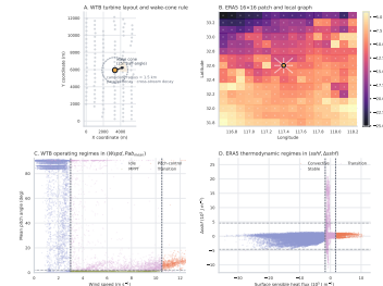
Fig. 1. Operating-decision context and physical regime anchors: (A) WTB layout with wake cone geometry (25° half-angle); (B) ERA5 patch with sensible heat flux; (C) WTB operating regimes in (Wspd, Pab_{\text{mean}}) plane with MPPT-to-pitch boundary; (D) ERA5 thermodynamic regimes in (sshf, \Delta sshf) plane.
