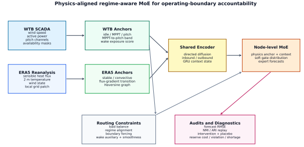
Interpretation: WTB tests a control-confounded turbine boundary; ERA5 is an observability contrast where the regime marker is visible. The routed model is evaluated as an accountability object, then linked to a frozen validation-to-test reserve diagnostic.
